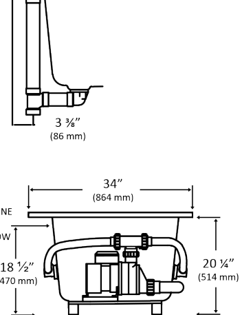
PLUMBING ROUGH-IN
