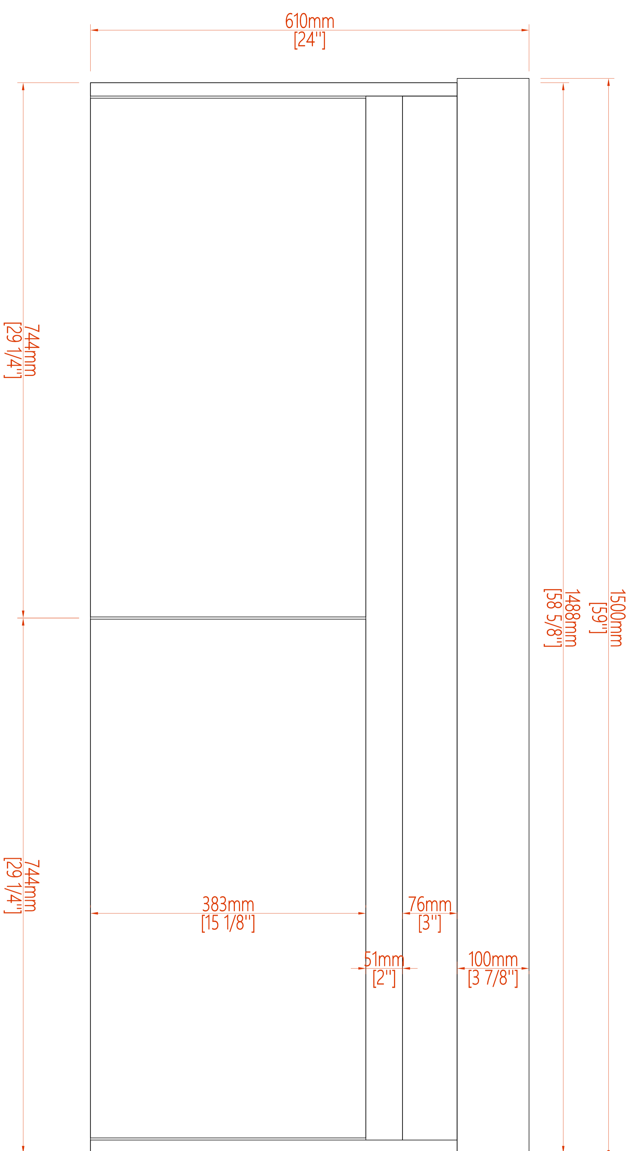
FRONT VIEW
