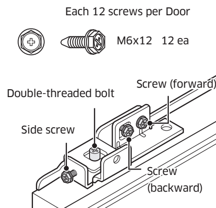
Panel-Adjustment Mechanism
