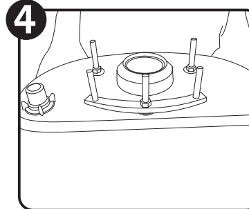
Qty 3 - 5/16 -18 retaining nuts 3 Tuercas de 5/16"
