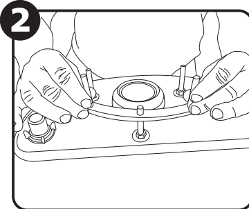
Corrosion resistant metal mounting bracket Platina en acero inoxidable calibre 16
