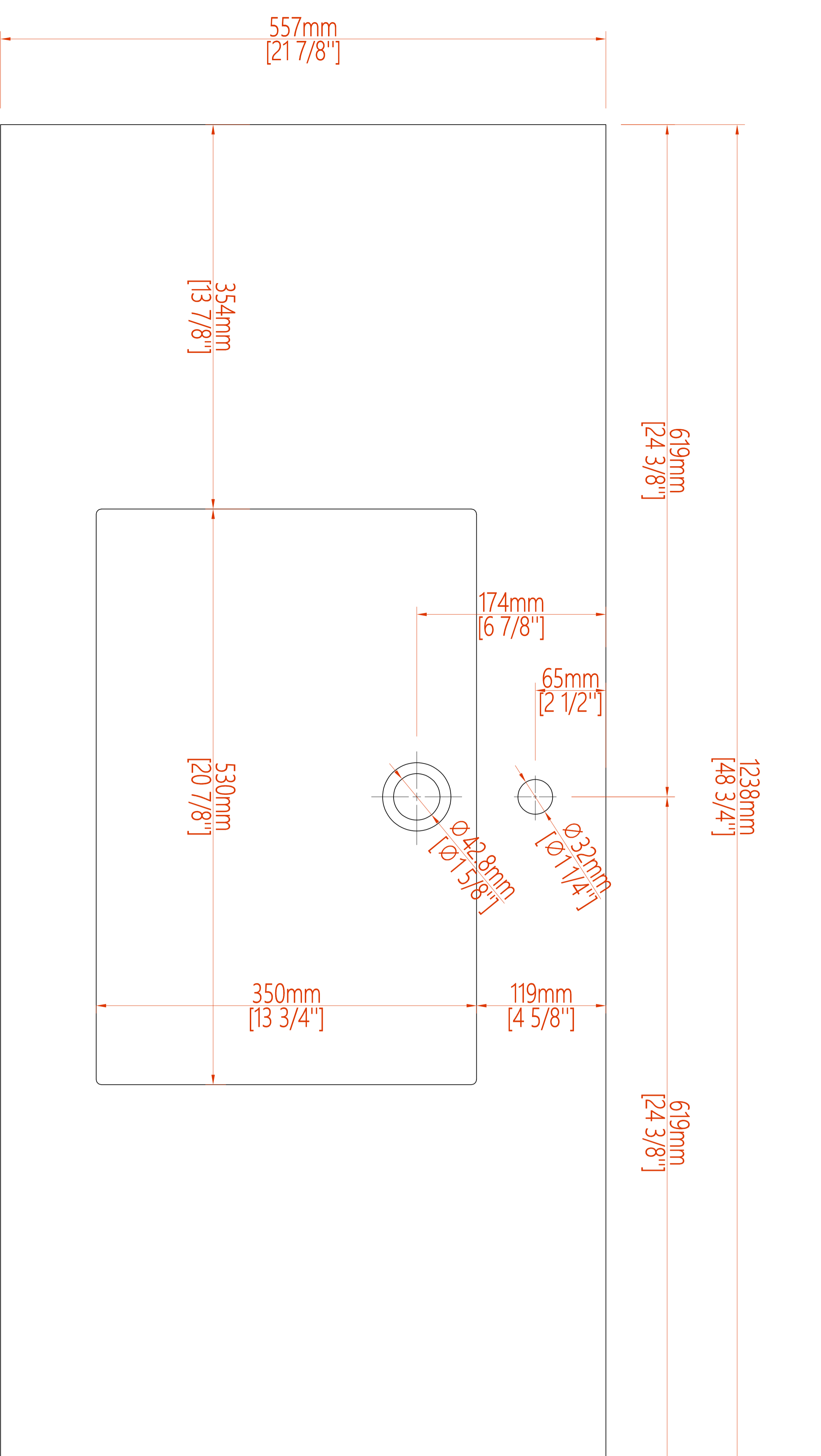
TOP VIEW
