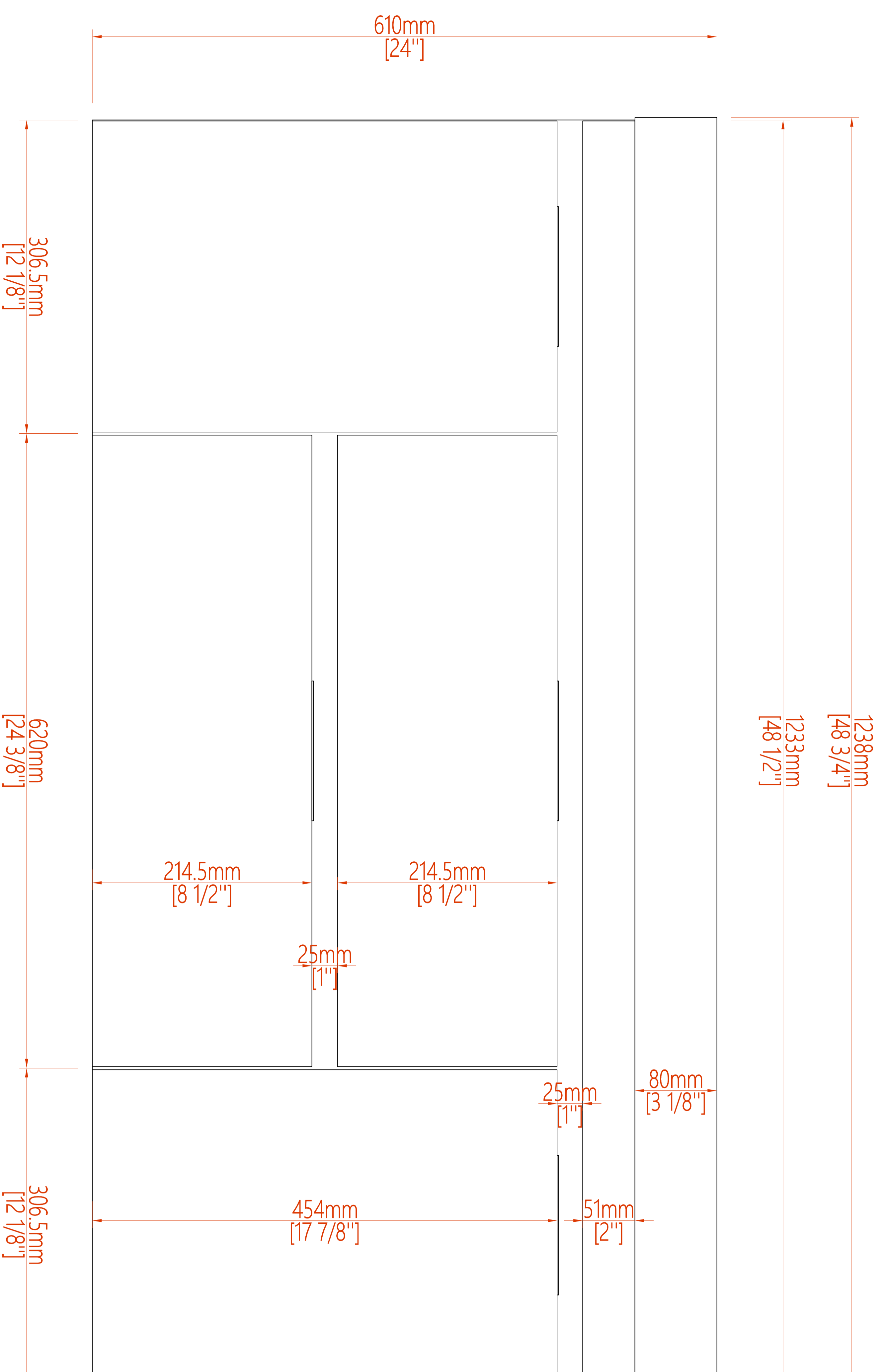
FRONT VIEW
