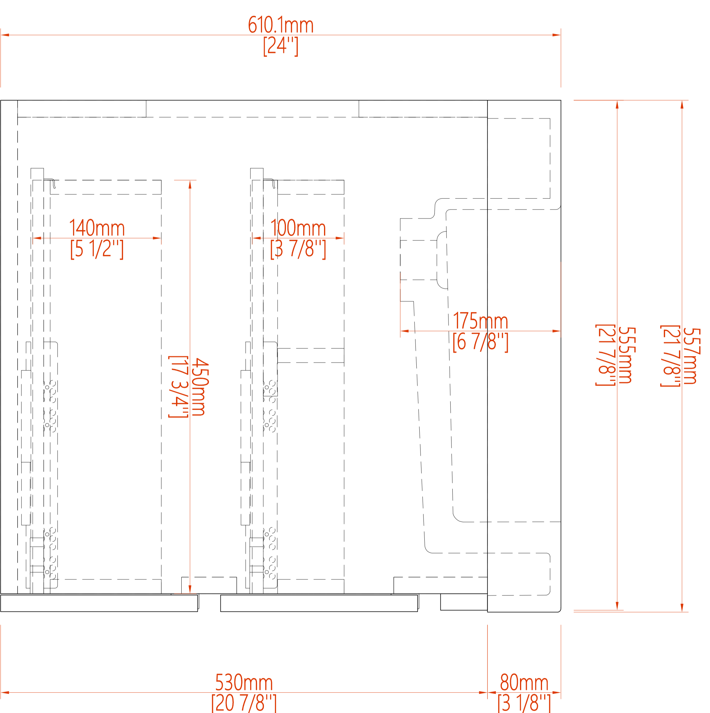
BACK VIEW
