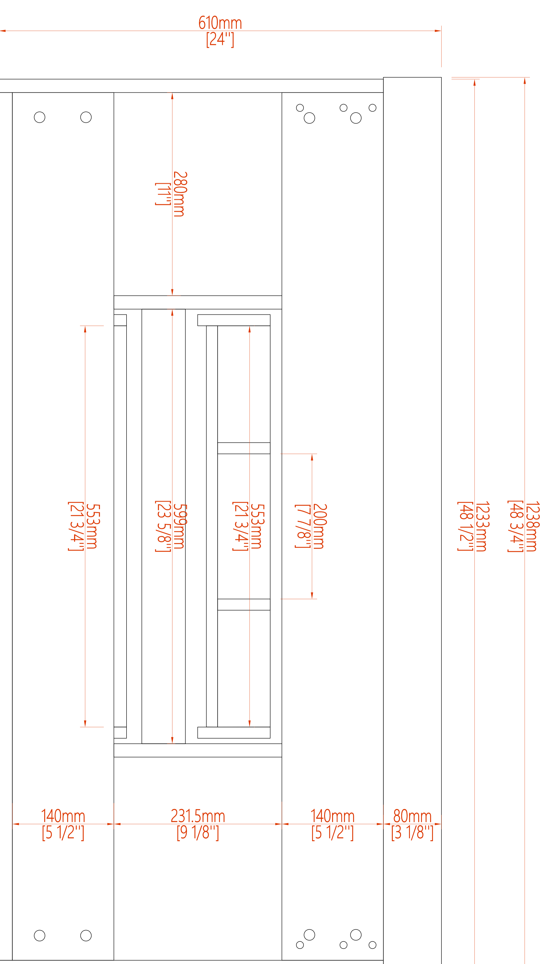
BACK VIEW
